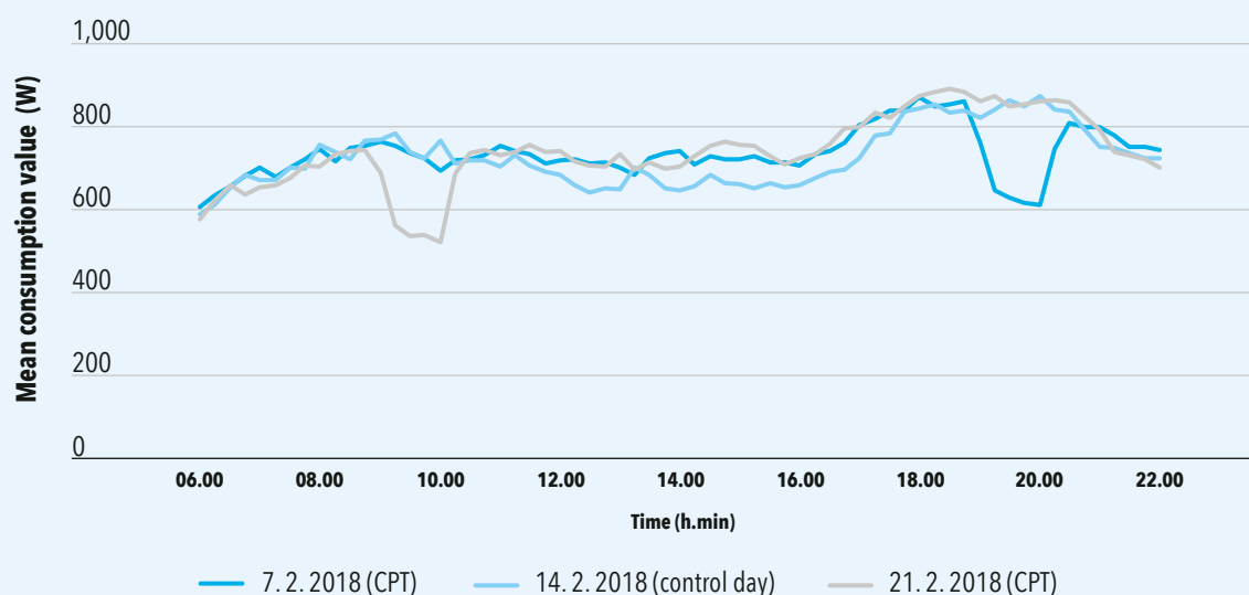
Figure 33: Course of daily load of pilot consumers of Elektro Maribor on the day of activations (on 7 and 21 February 2018) compared to the control day (14 February 2018)
